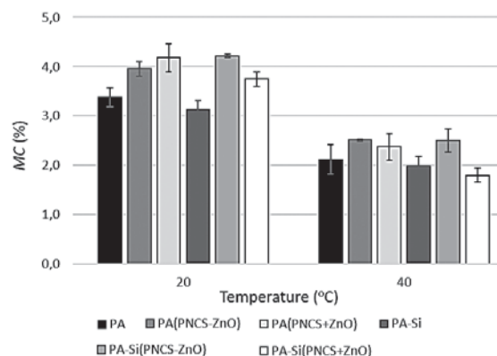
Figure 3: Moisture content, MC, of the untreated and differently coated samples obtained after preconditioning at 65% R.H. and 20 °C and 40 °C
