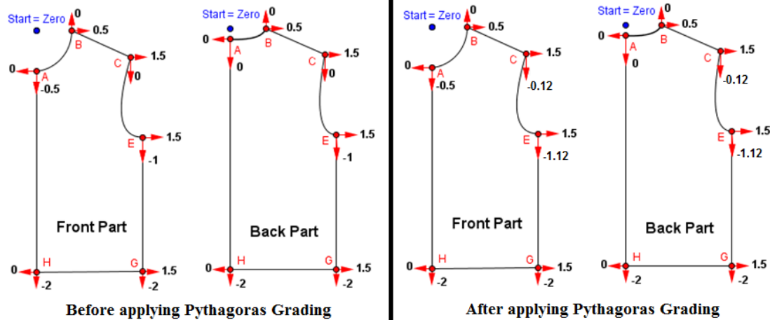
Figure 11: Grading increment of pattern pieces of T-shirt body parts (spec B) before and after Pythagoras grading (L size as base size)
