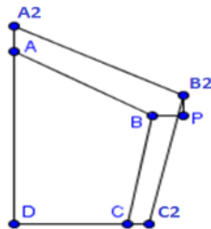
Figure 25: Points to calculate grading increment for the pattern pieces of T-shirt sleeve pattern of spec A (method 2)
