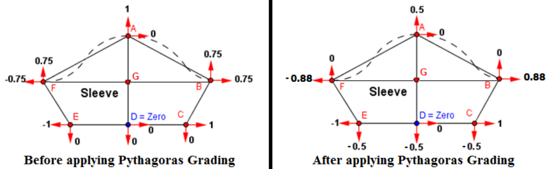
Figure 24: Grading increment of pattern pieces of T-shirt sleeve spec A (method 1) before and after applying Pythagoras grading
