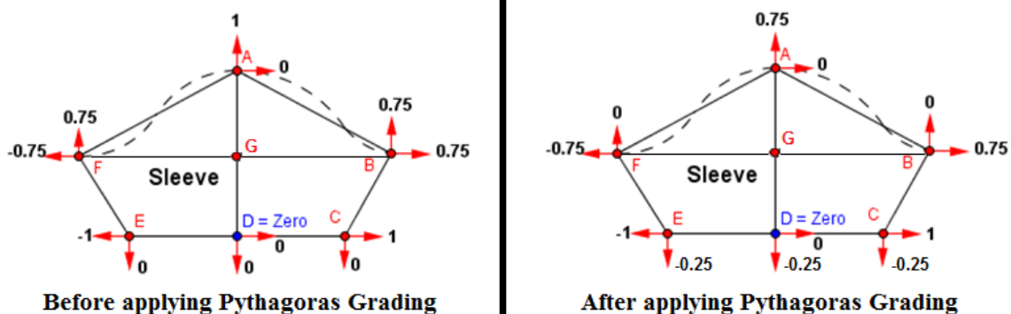
Figure 22: Grading increment of pattern pieces of T-shirt sleeve of spec B before and after Pythagoras grading
