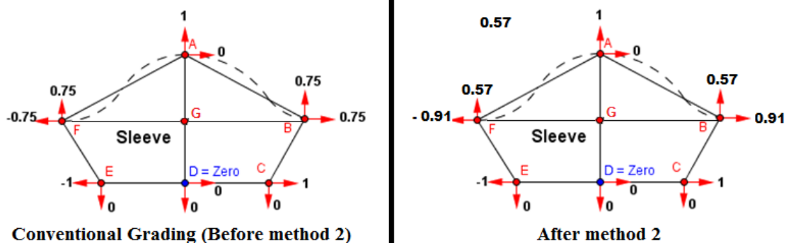
Figure 26: Grading increment of pattern pieces of T-shirt sleeve spec A before and after applying method 2
