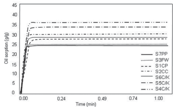
Figure 13: Sorption of diesel oil by the nonwovens with time
