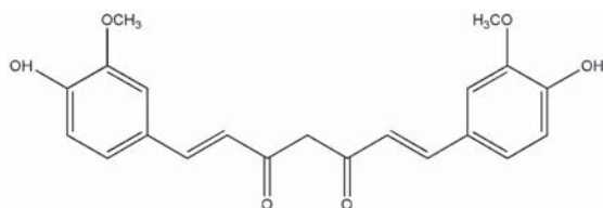
Figure 1: Chemical structure of curcumin (keto form) [14]
